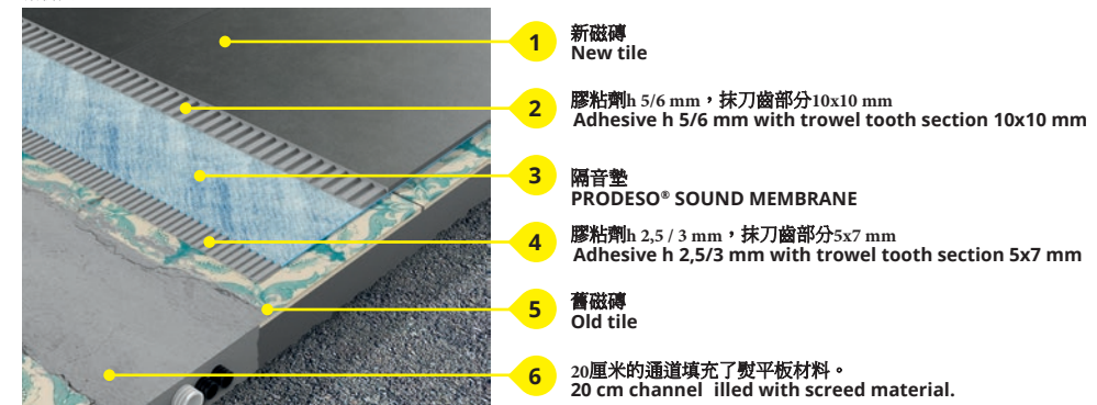
LAYING'S SECTION OF PRODESO® SOUND SYSTEM 剖析圖
