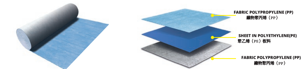
LAYING'S SECTION OF PRODESO® SOUND SYSTEM 剖析圖
